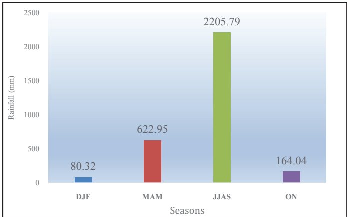
Figure 9: Mean Seasonal distribution nearby Barsa watershed
