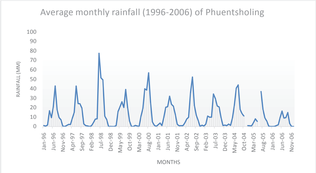
Figure 11: 1996-2006 average monthly rainfall at Phuentsholing
