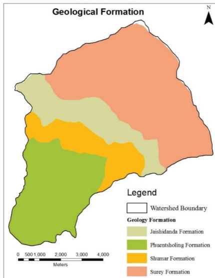
Figure 5: Geological map of the watershed
