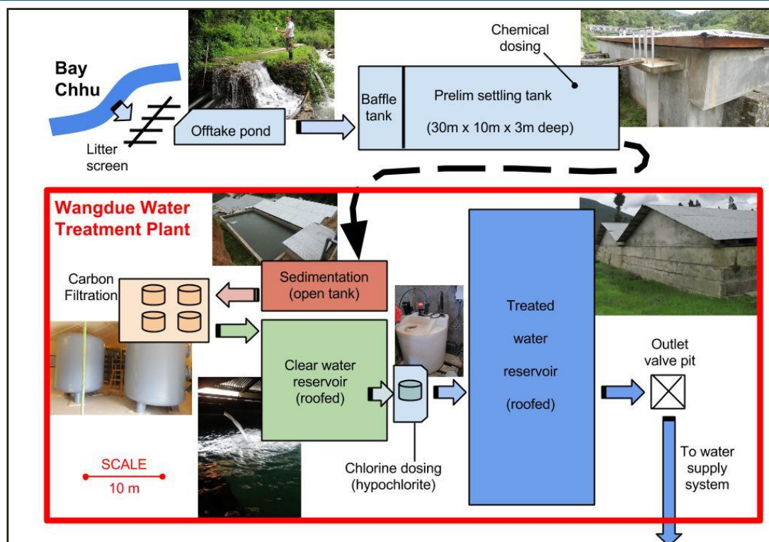
Fig. 10: Water treatment system
