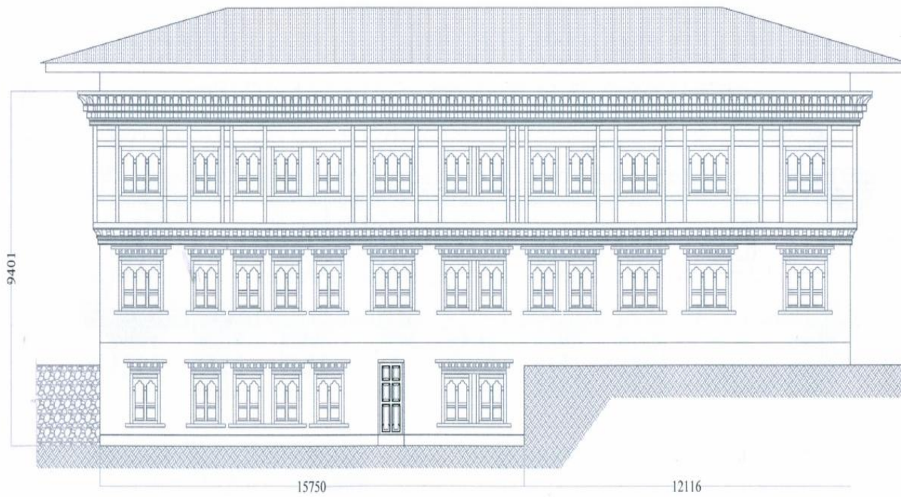
ELEVATION C
